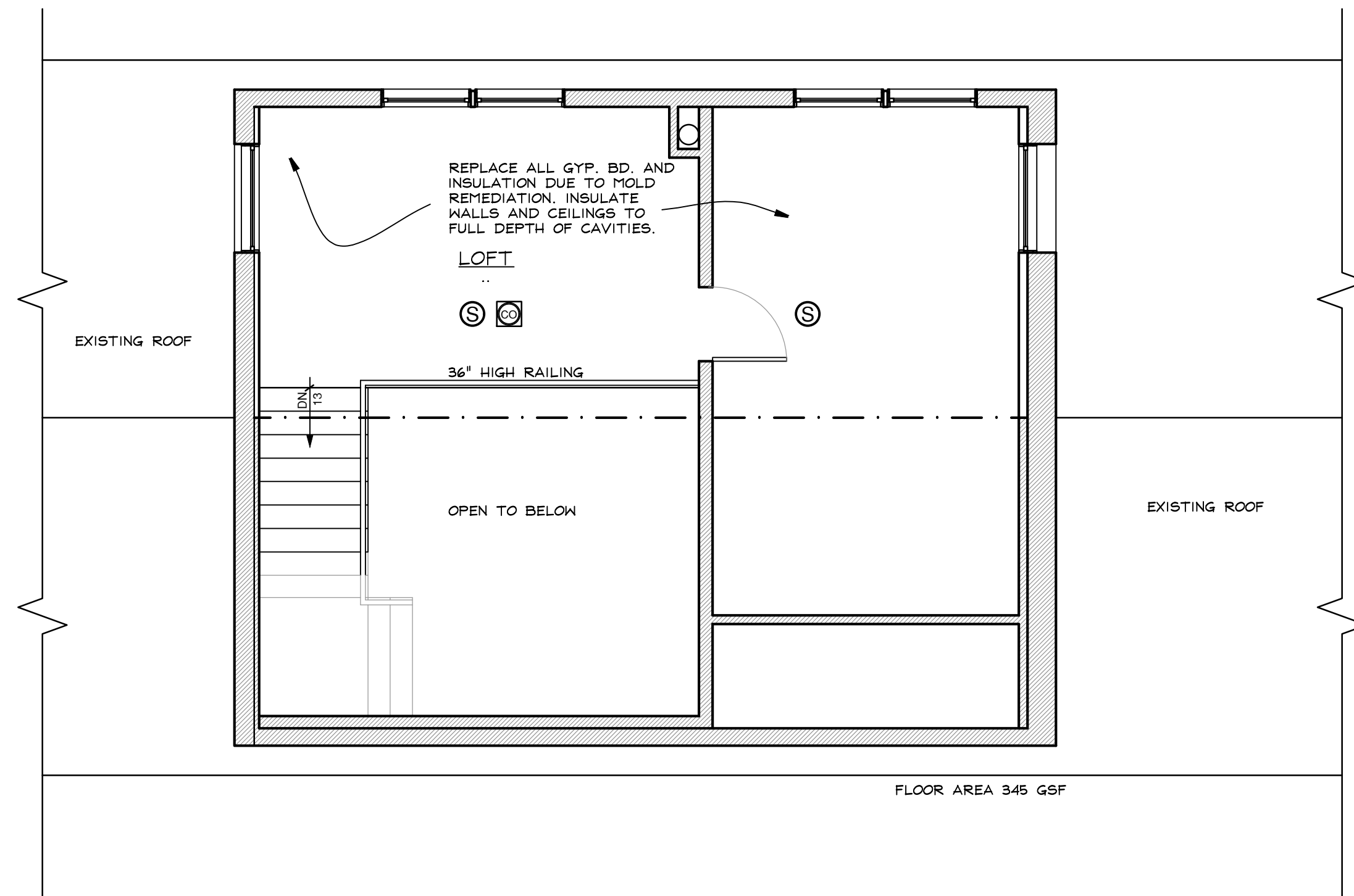
1 SECOND FLOOR PLAN 1/4" = 1 FOOT
