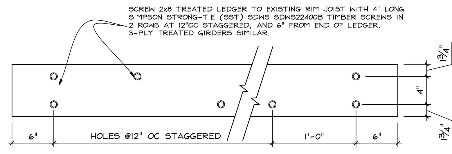
B LEDGER FASTENING DETAIL A3 1 1/2" = 1 FOOT
